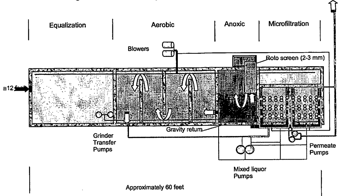
Figure 15 - General Layout of Membrane Bioreactor
